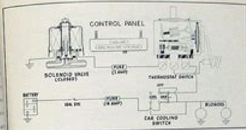
Fig. 8b. Information Wiring Diagram of Control Circuit
