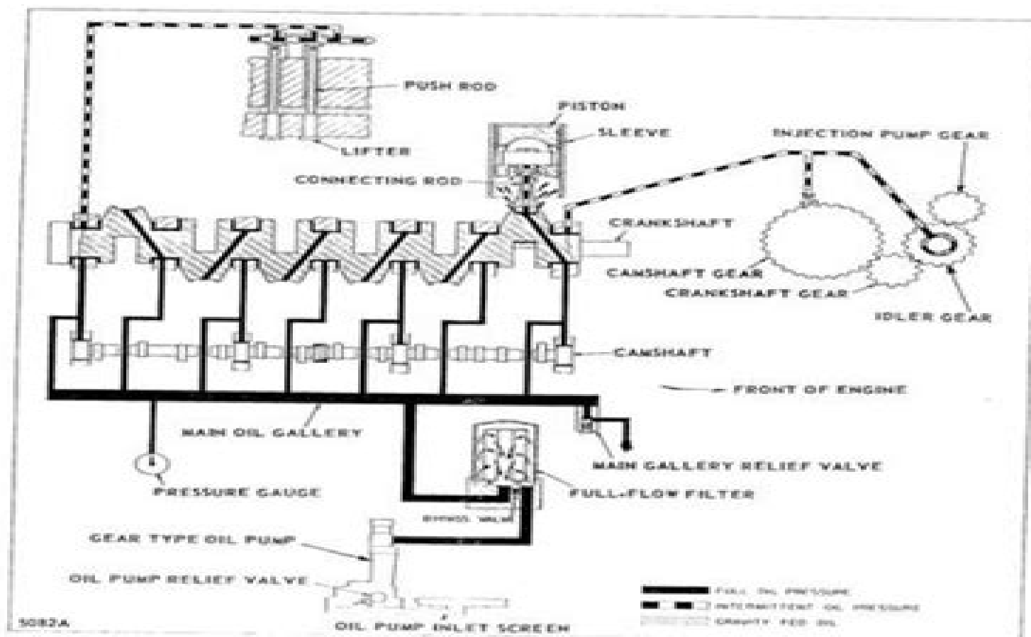
Fig. B10-15-3 Direct Engine Lubrication
