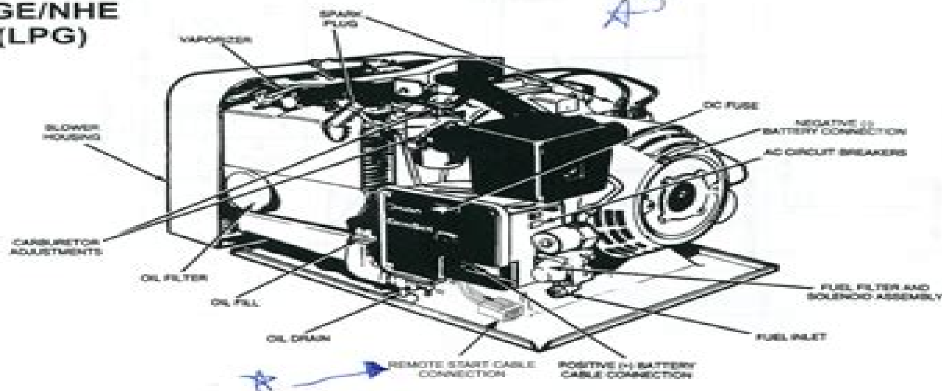
FIGURE 1-1. TYPICAL EMERALD PLUS GENERATOR SETS
