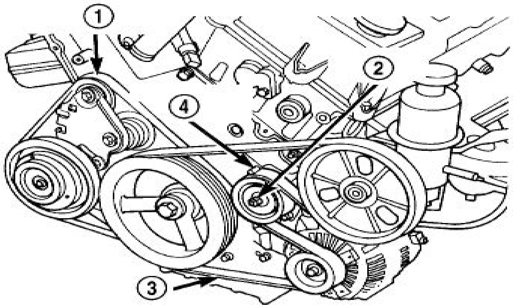
Fig. 45 Accessory Drive Belts
