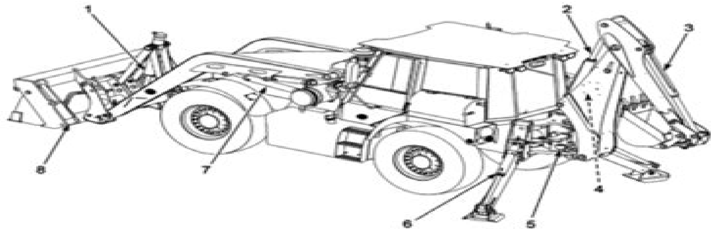
Figure 6. Hydraulic System
