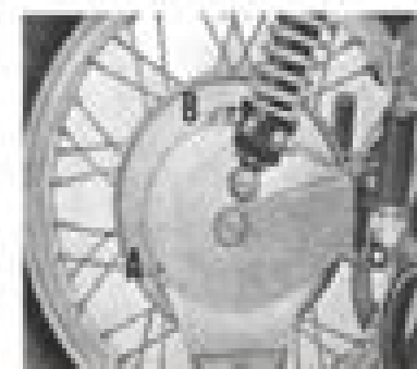
Rear wheel drive oil level, filler, and drain plugs (V750 and V100)
