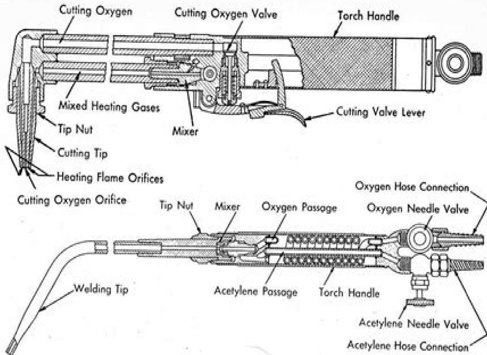
FIGURE 149. Oxy-acetylene cutting torch (top), oxy-acetylene welder (bottom).
