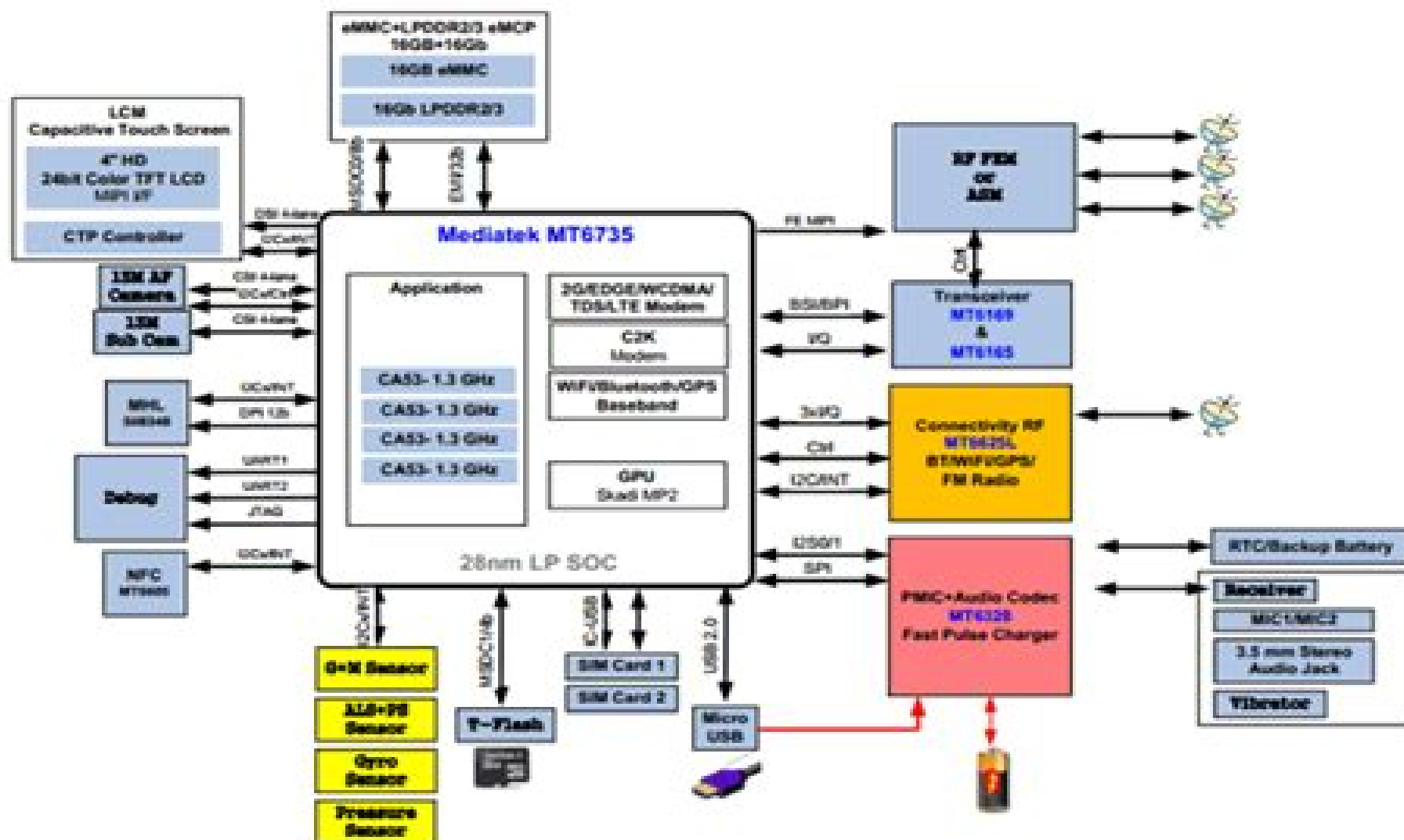
Figure 1-1. High-level MT6735 functional block diagram
