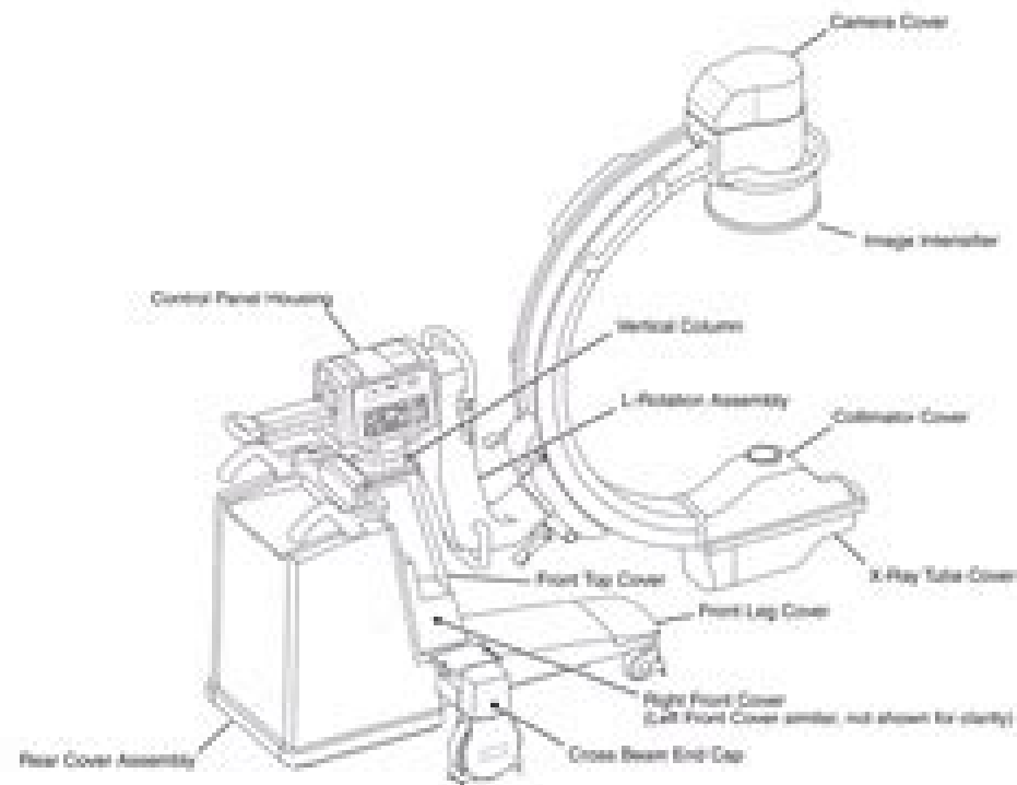
Standard C-Arm Subsystem Major Assembly and Control Locations
