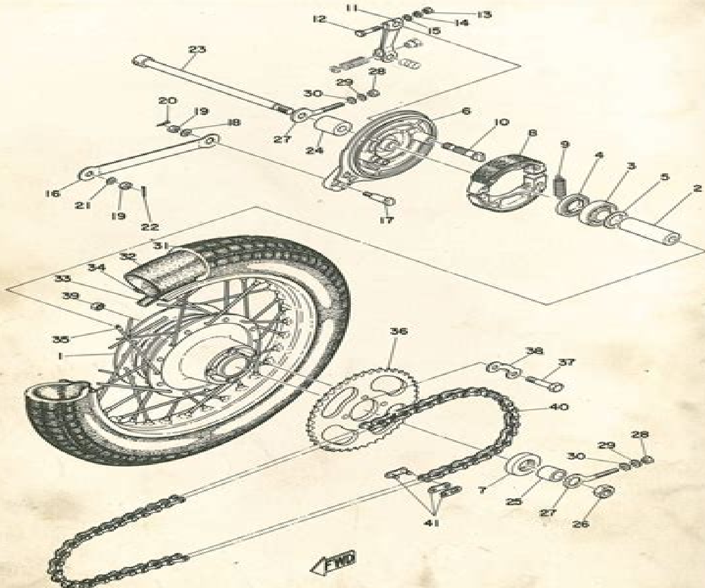
Fig. 24 REAR WHEEL
