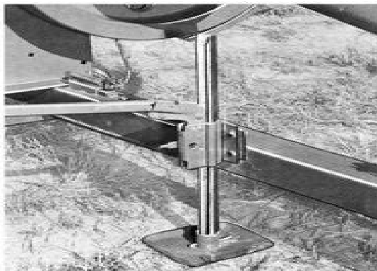
Fig. 10 - Leveling Jack
