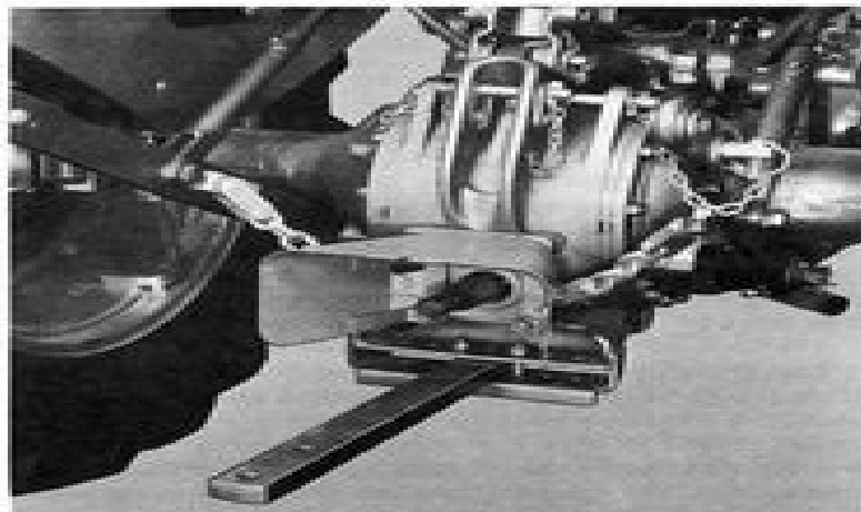
Fig. 9 - Universal Drawbar with PTO Adapter Installed
