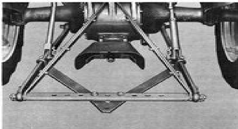
Fig. 7 - Extension "V" Drawbar with PTO Adapter (12'')
