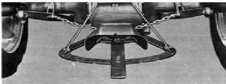
Fig. 8 - Swinging Drawbar with PTO Adapter Installed
