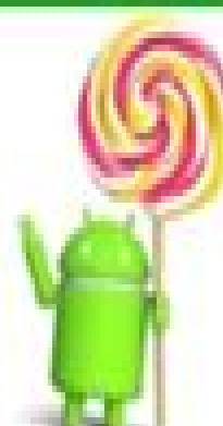
Lollipop Android 5.0
