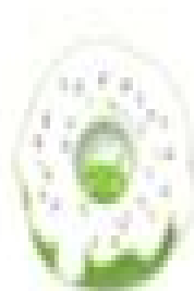
Donut Android 1.6
