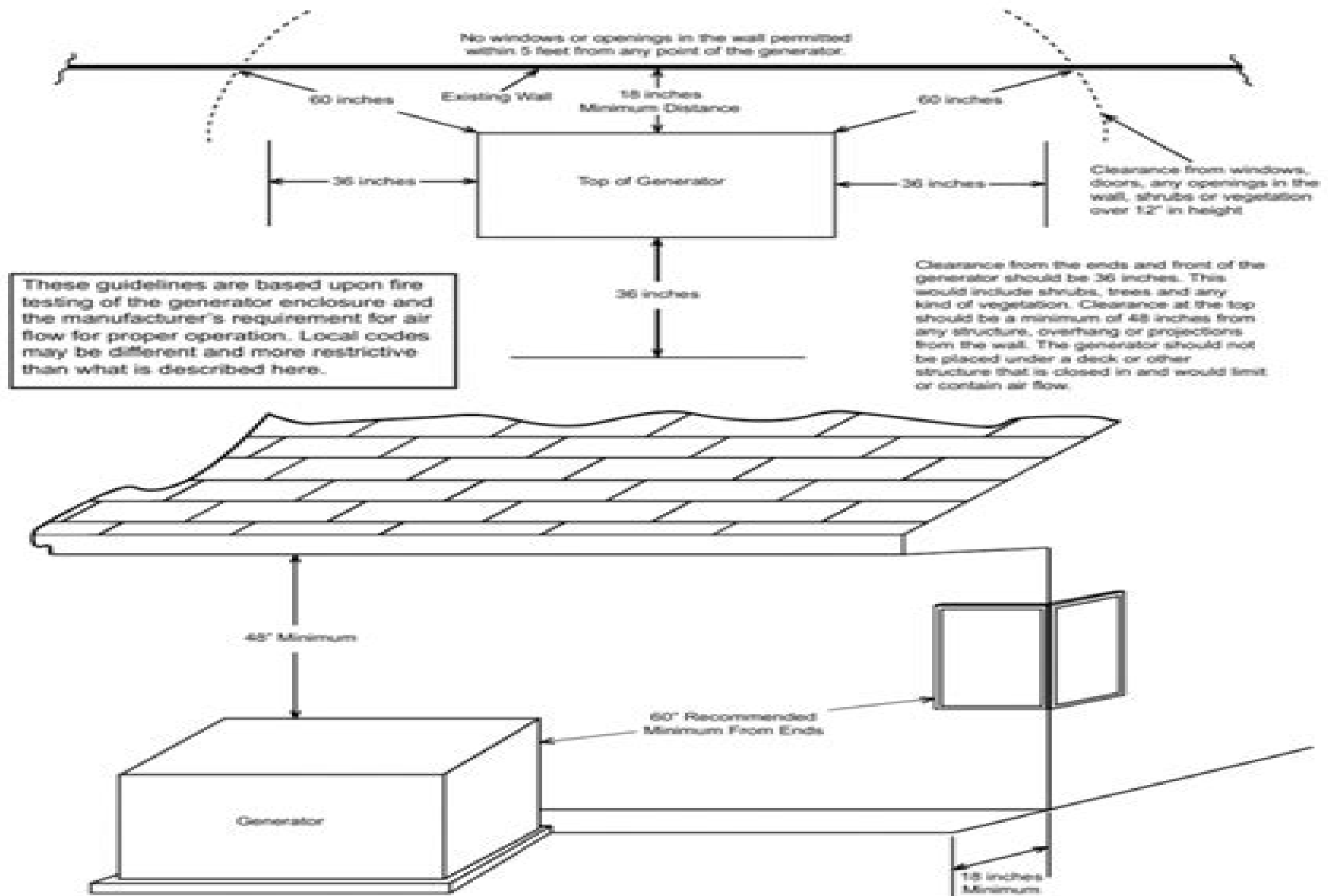
Figure 1.10 – Installation Guidelines
