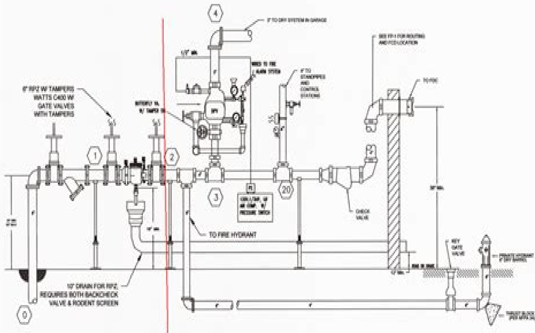
RISER SCHEMATIC NO SCALE
