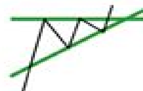
Ascending Triangles
