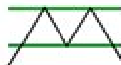
Double Top
