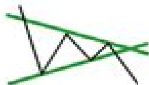
Symmetrical Triangles
