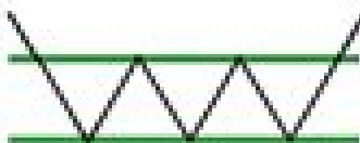
Triple Bottom
