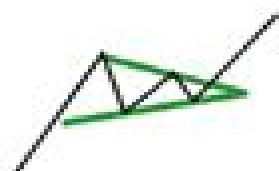
Pennants
