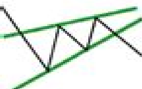
Wedge Continuation
