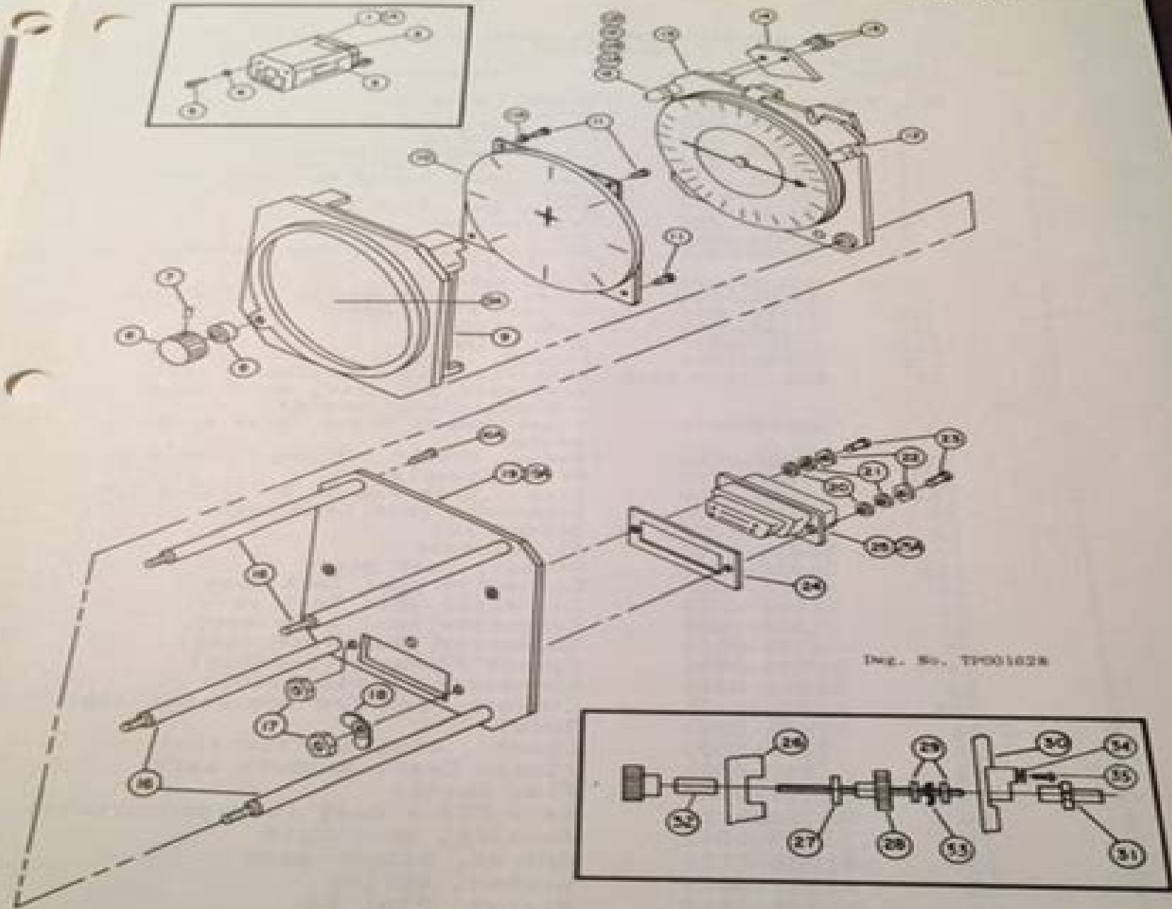
FIGURE 6-6 ID-841 INDICATOR
