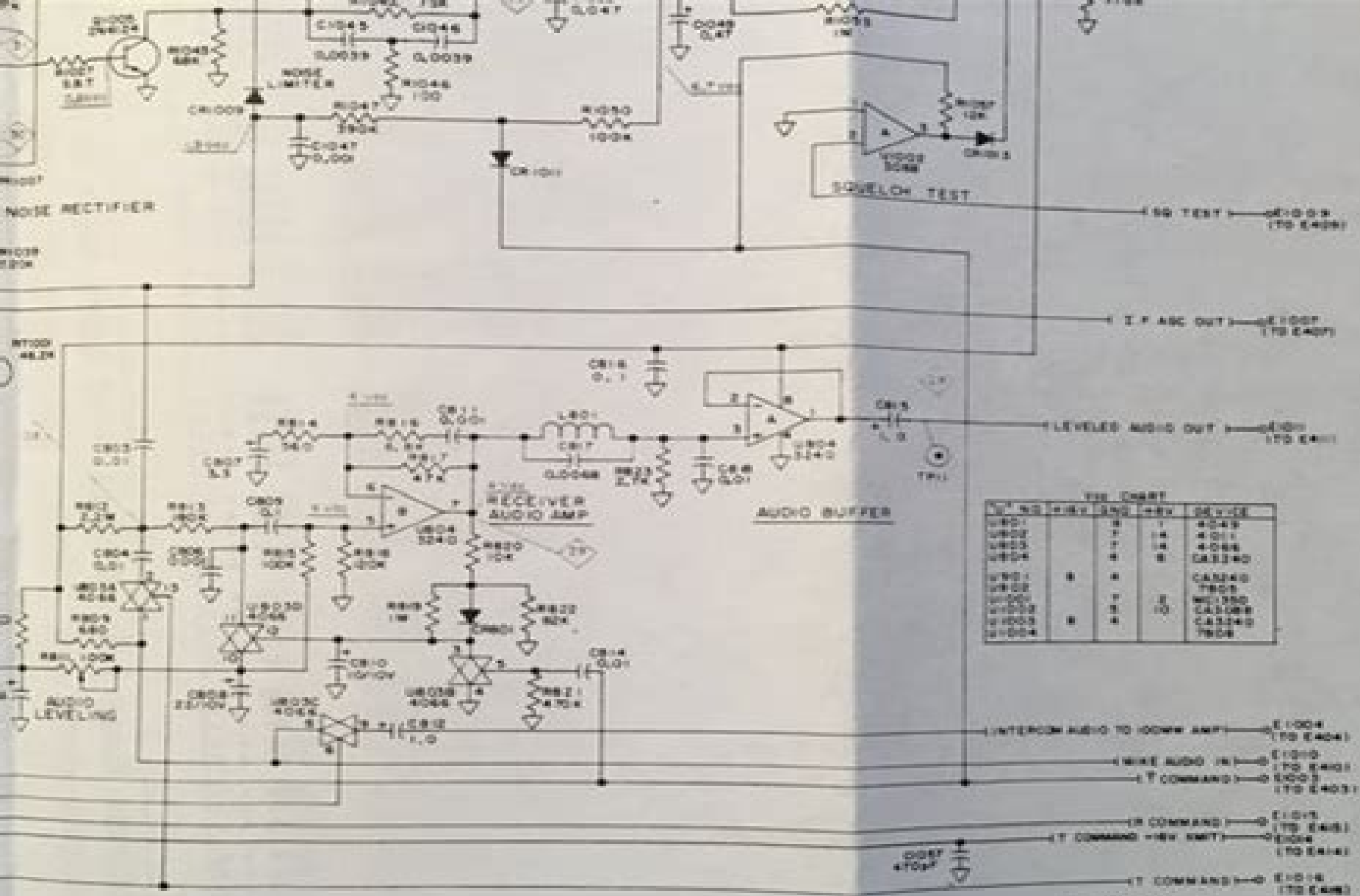
FIGURE 6-5. RECEIVER PC BOARD (sheet 2 of 2)
