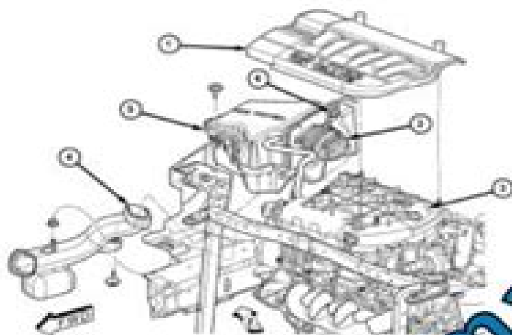
Fig. 4 AIR INTAKE SYSTEM
