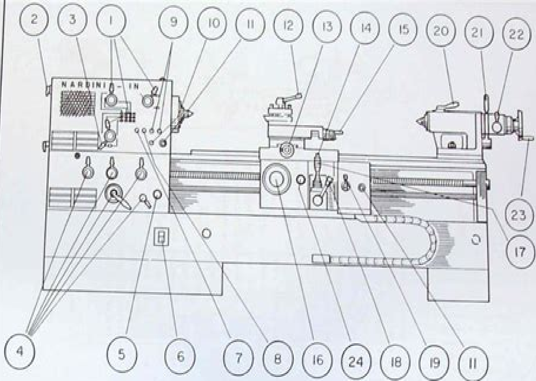
FIG. 5 LATHE CONTROLS
