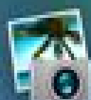
iPhoto
