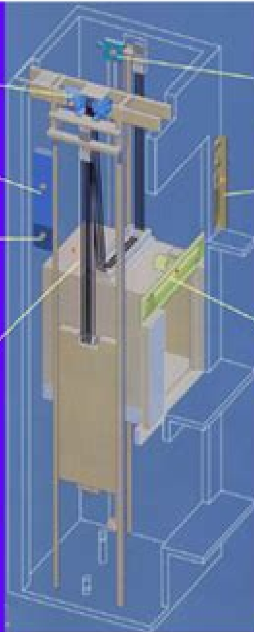
Diagram of OTIS Gen2 Lift
