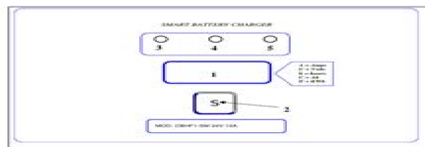
FRONT PANEL OF BATTERY CHARGER MODEL CBHF1-SM
