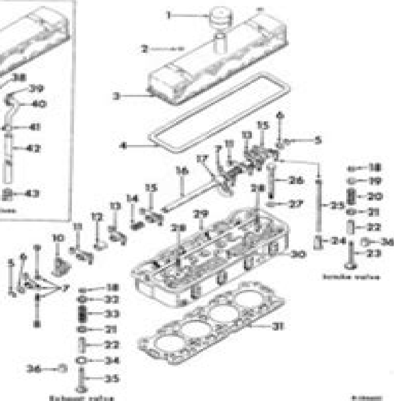
Exhaust valve
