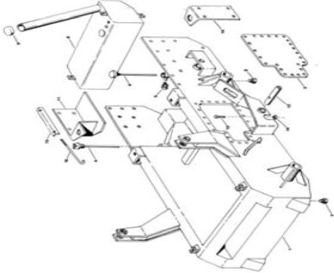
MAIN FRAME & FUEL TANK
