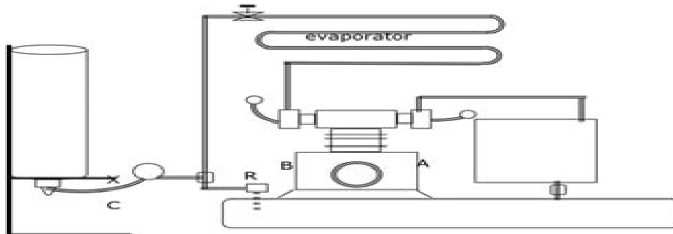
Gambar 7. Pengisian bahan pendingin sistem high side charging
