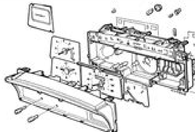
Fig. 12-8 Exploded diagram of front-left instrument panel
