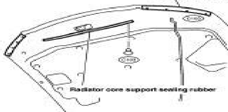
① Radiator core support sealing rubber
