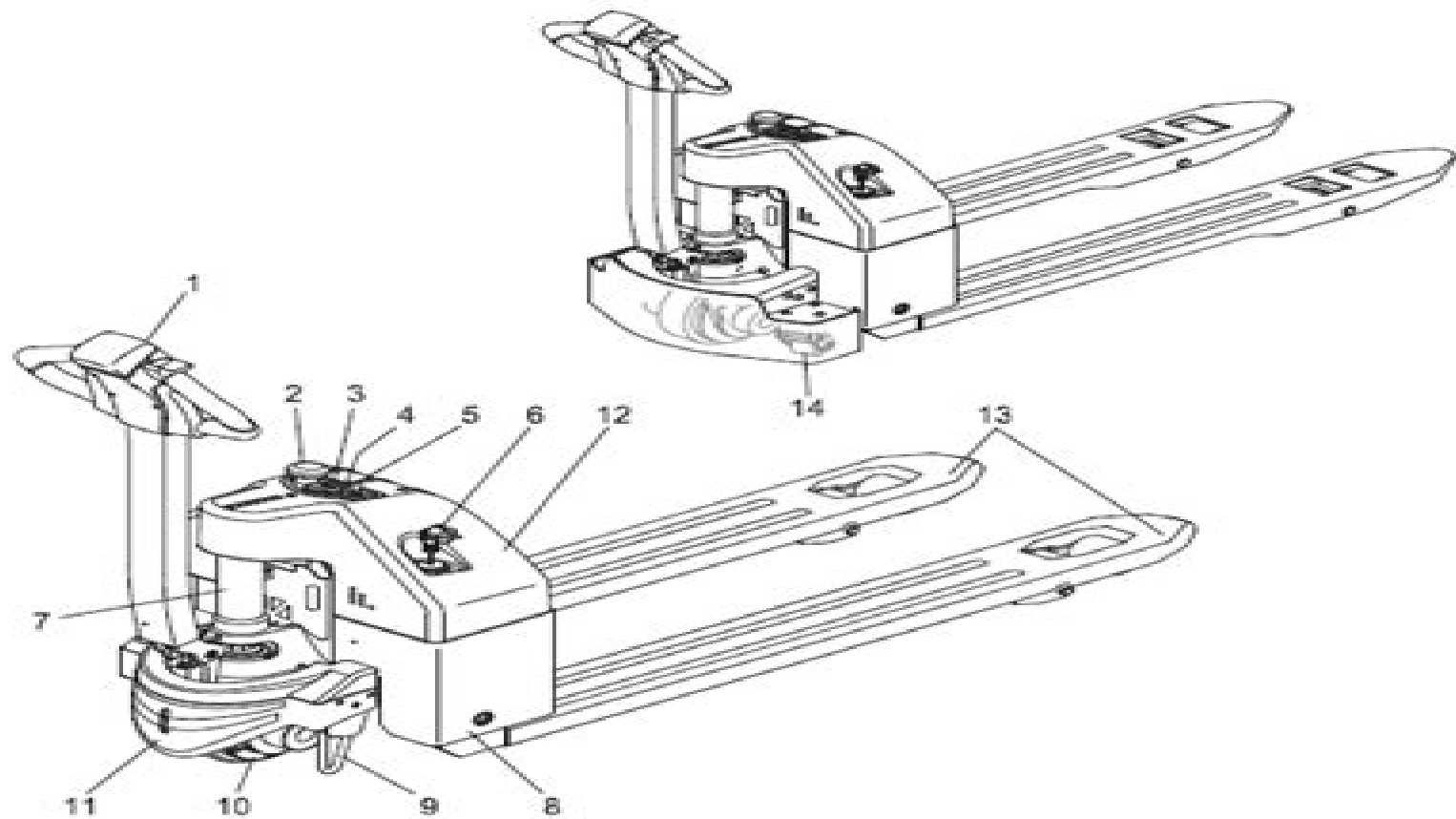
Figure 1-2 Lift Truck
