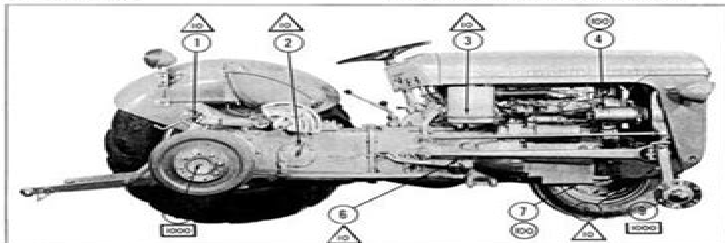
Lubrication Chart
