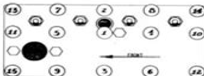
Head nut tightening sequence
