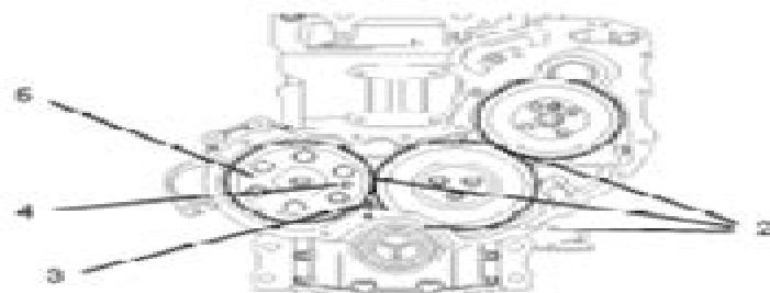
Illustration 119 Typical example (Delphi fuel pump drive gear)
