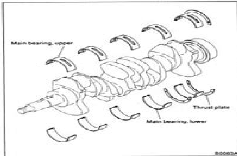
(b) Main Bearing
