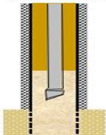
OPEN ENDED (SUSPENDED) TUBING PRODUCTION
