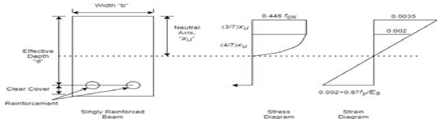
RCC Rectangular Beam with Stress & Strain Diagrams as per Limit State Method
