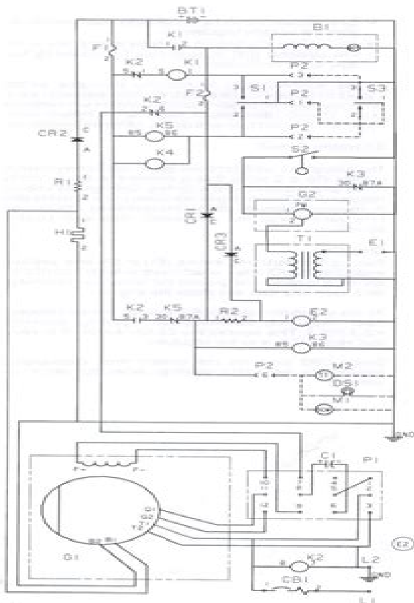
FIGURE 7-1. SCHEMATIC - 60 HERTZ
