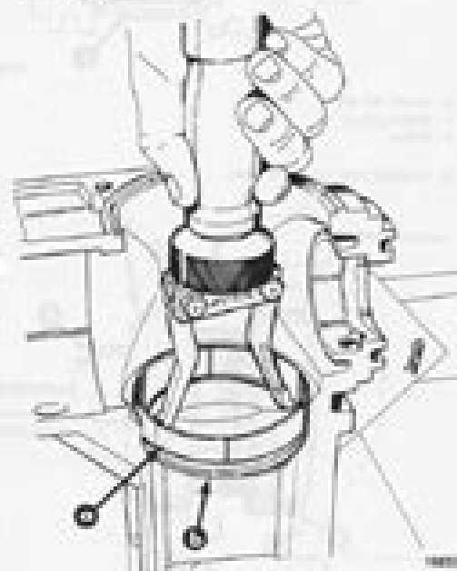
a - Bearing Cap b - Drive
