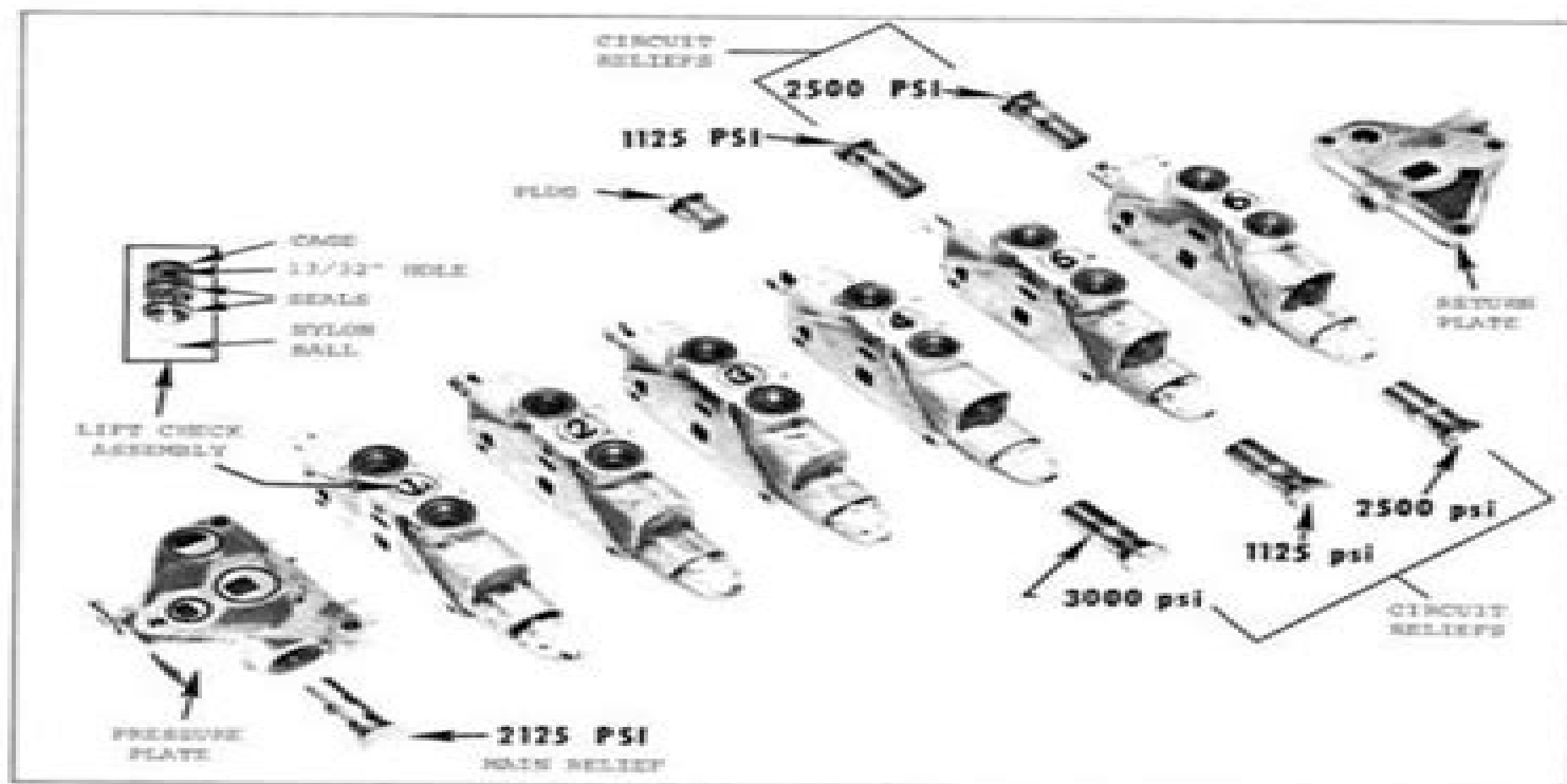
Fig. 11 — Identification of Valve "Working Sections" — MF Part No. 705 937 M92
