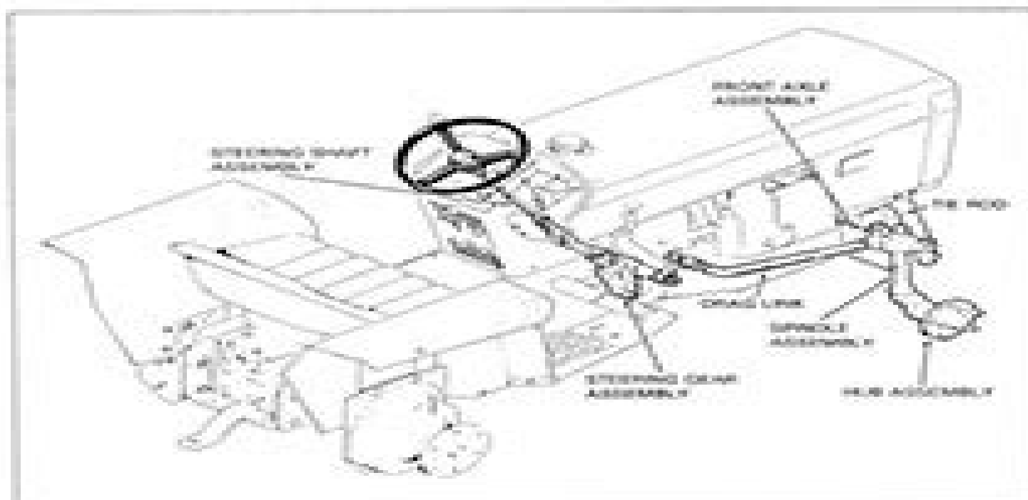
Figure 85. Steering and Front Axle Assemblies
