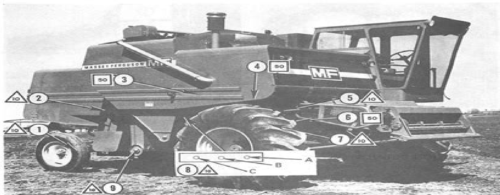
Fig. 107 — Lubrication — Right-Hand Side
