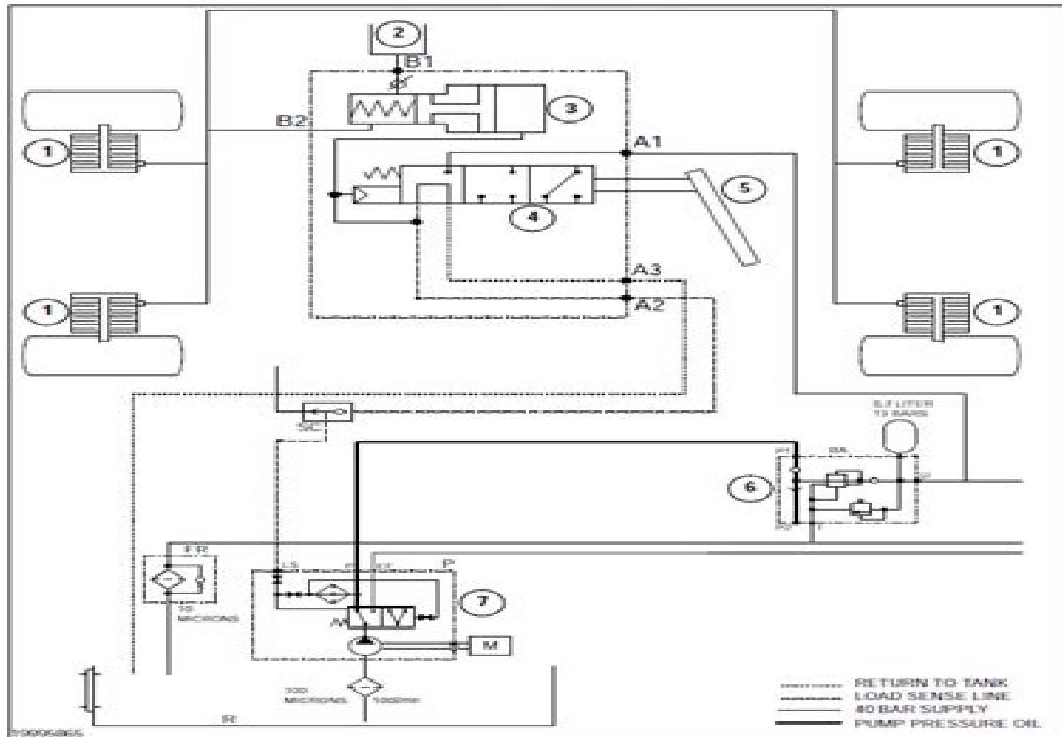
Brake System Schematic
