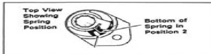
Figure 5-13. Choke Lever With Cap Removed.
