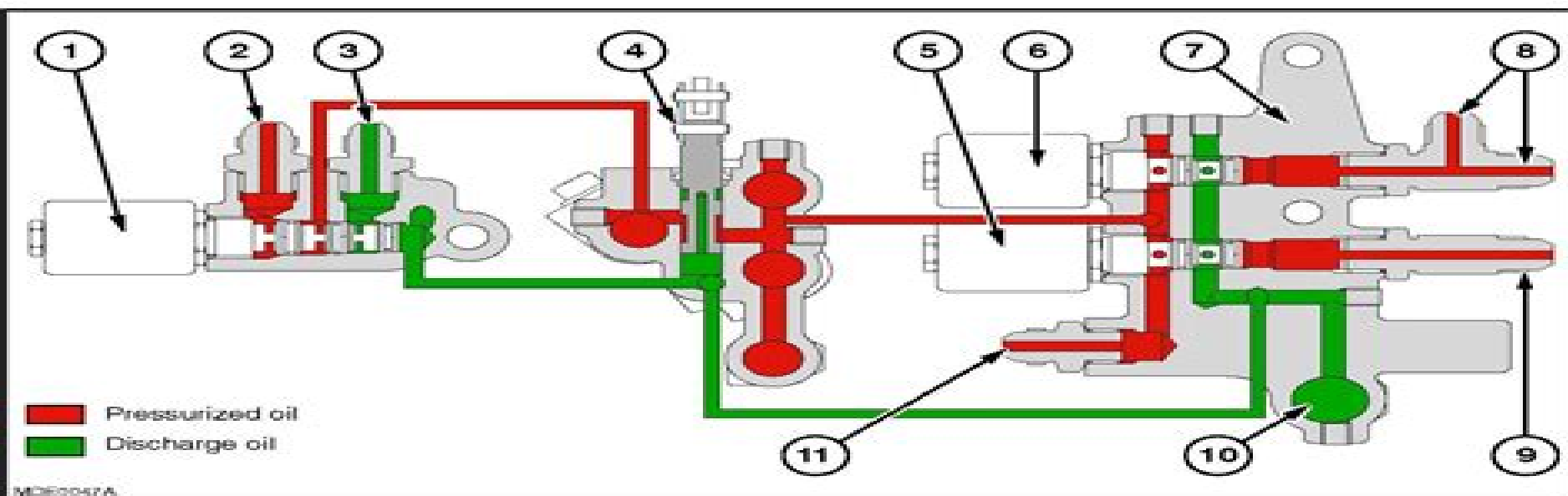
Services control valve hydraulic diagram (points 2 and 3 pages 13 and 15)
