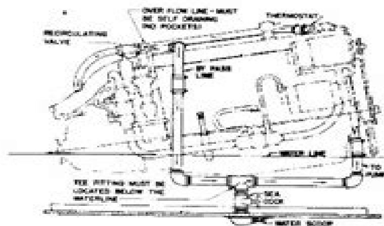
Fig. 4A—Piping Diagram for Engines with Dual Unit Thermostat. Pipe size for all external lines must never be smaller than the pump intake size
