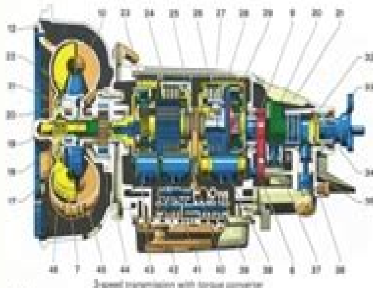
Fig. 2 3-speed transmission with torque converter
