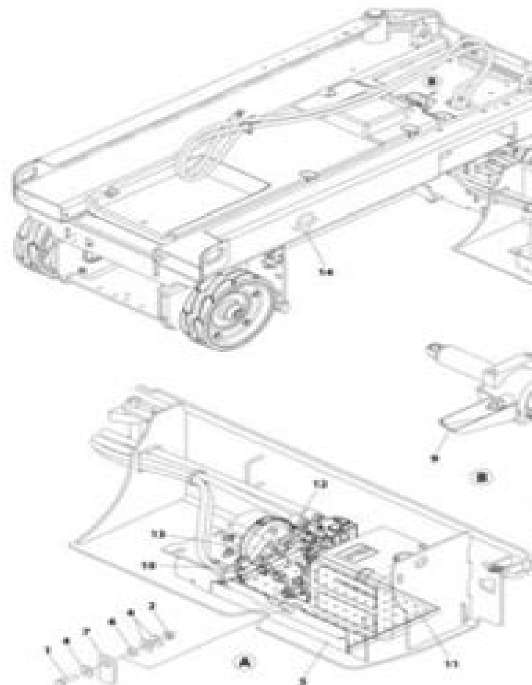
FIGURE 2-3. CLEANGUARD INSTALLATION (MACHINES WITH SN ST
