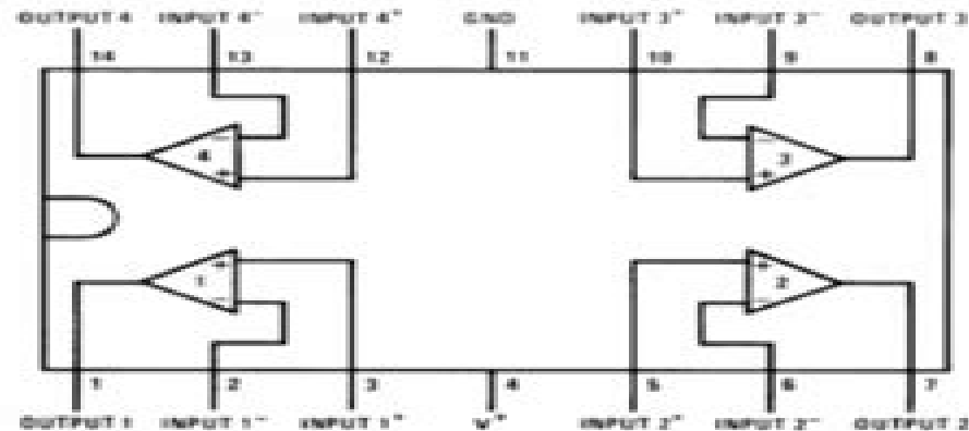
Figure 1. Pinout for the LM324.
