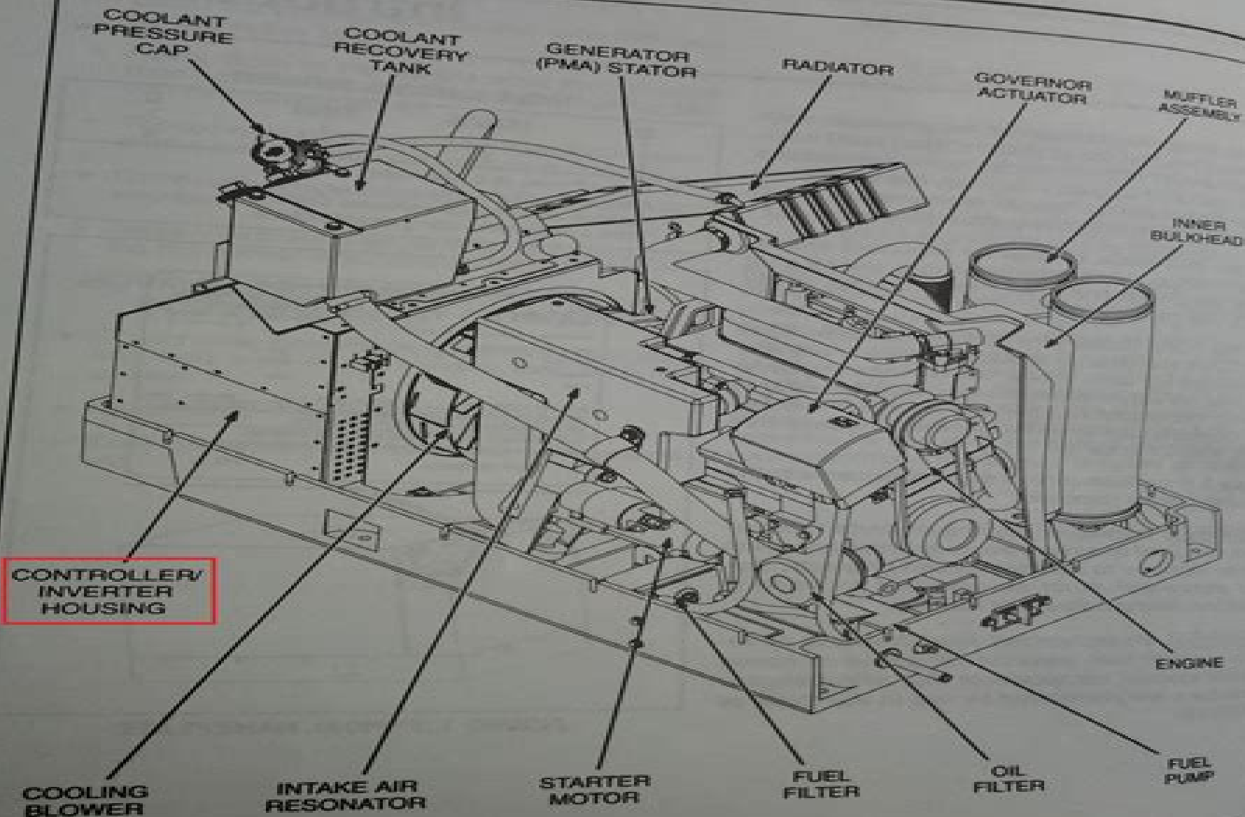
FIGURE 2. TYPICAL GENSET WITH HOUSING PANELS REMOVED
