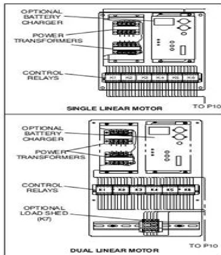
FIGURE 2-13. CONTROL PLATE
