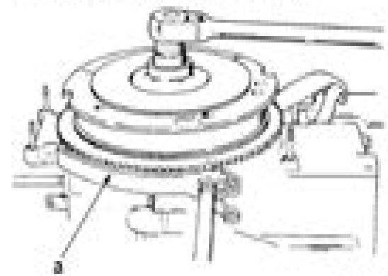
a - Flywheel Holder (91-52344)
