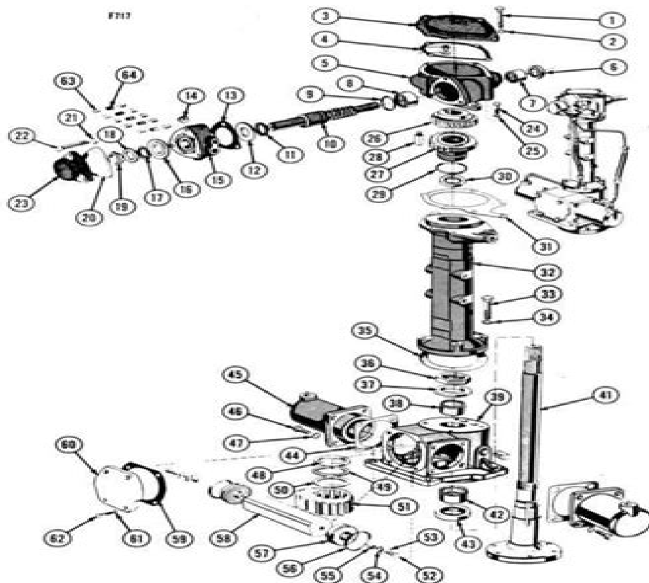
Fig. 3 - Power Steering Details and Relative Location of Parts
